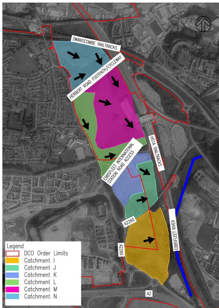
Figure 17.10: Kent Project Site (Access Road) – Existing Catchments (prepared by WSP).
